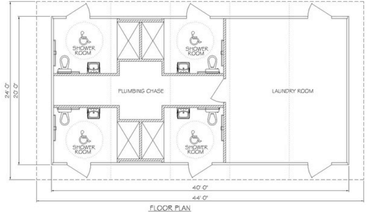
FLOOR PLAN
